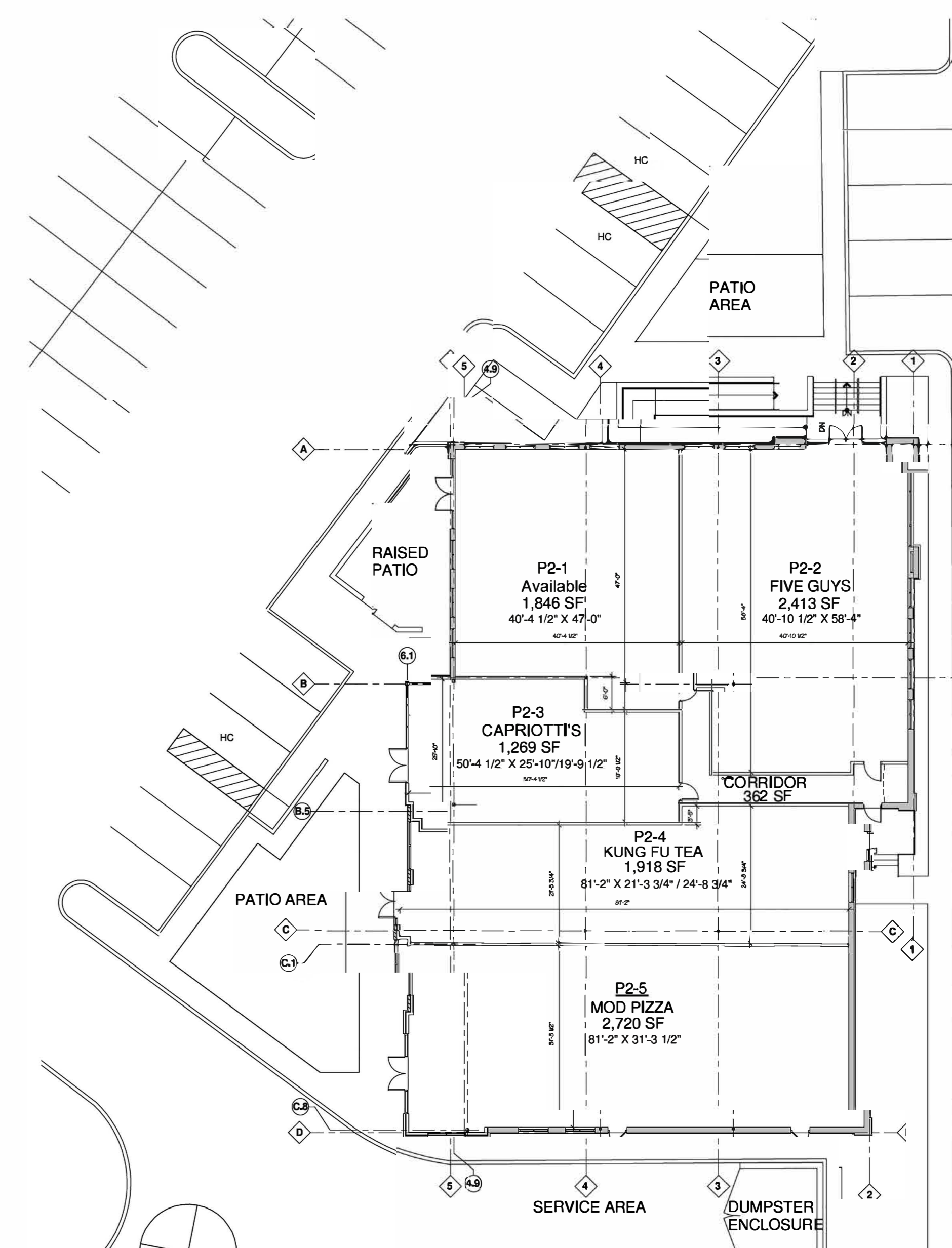
FLOOR PLAN - PAD P2
